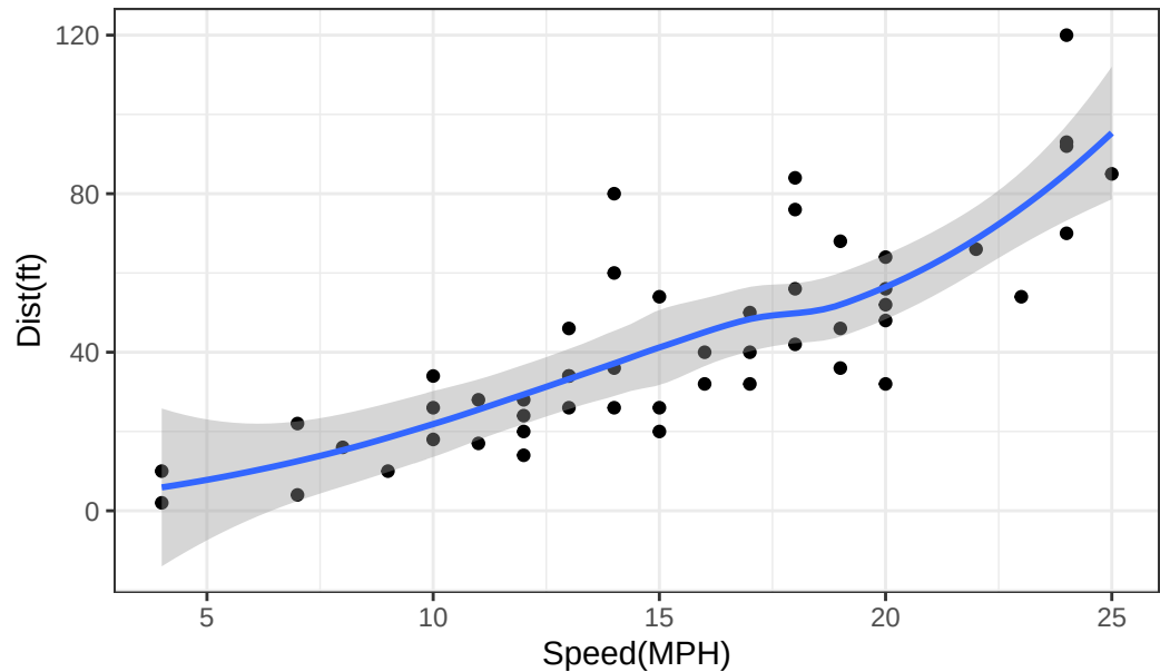
Stopping Dist of old cars
